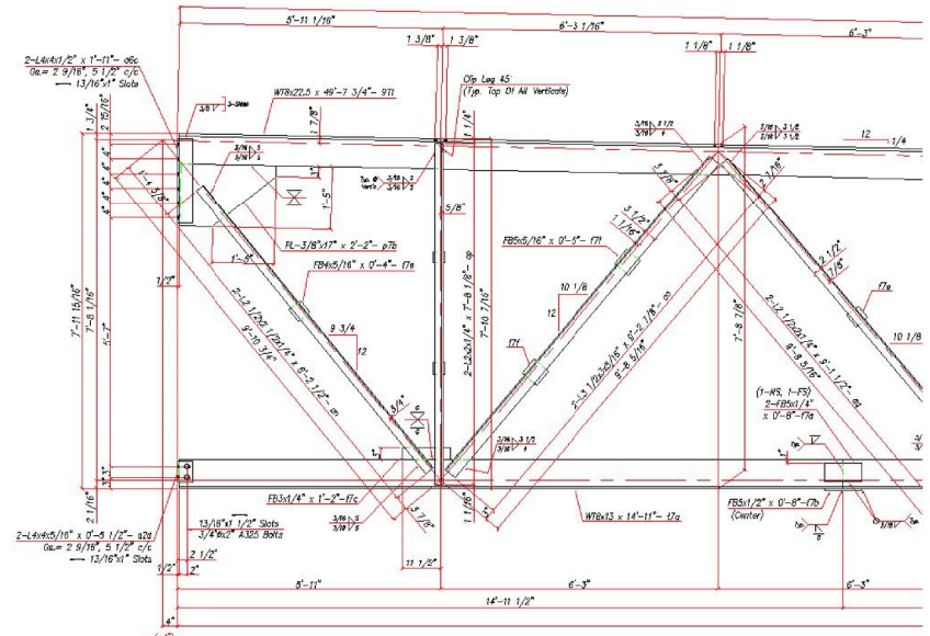
Truss Sample - Nissan Addition - Smyrna, TN
